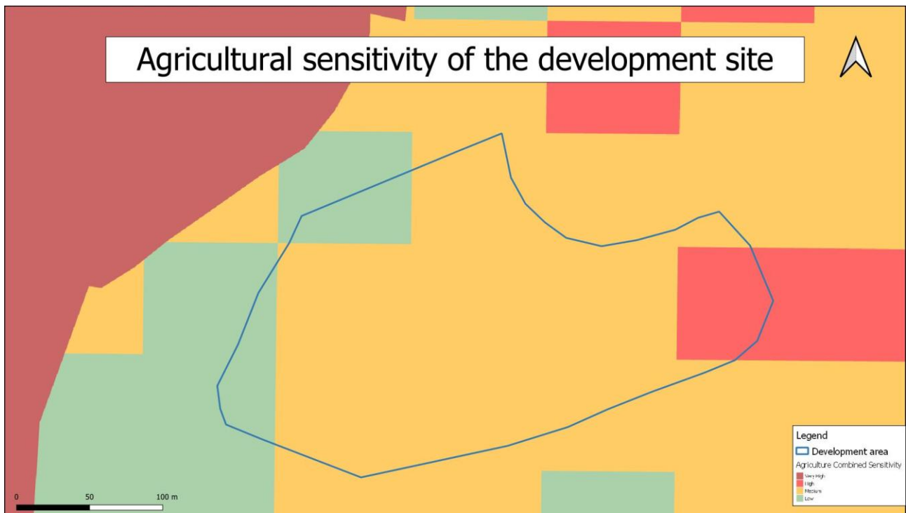
Figure 2. The assessed area overlaid on agricultural sensitivity, as given by the screening tool.
